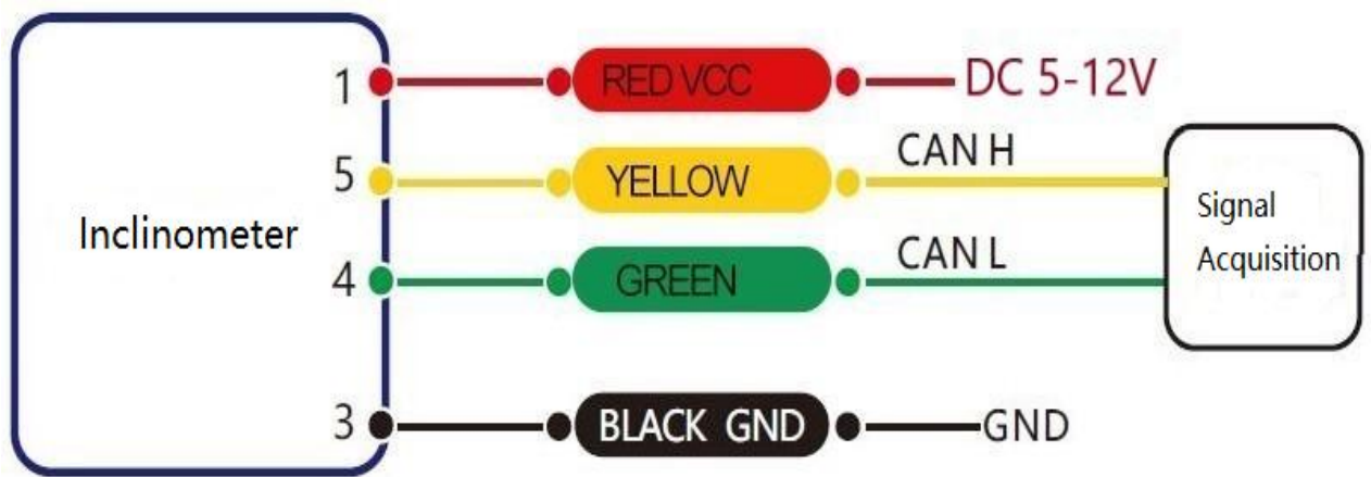
CAN bus connection diagram
